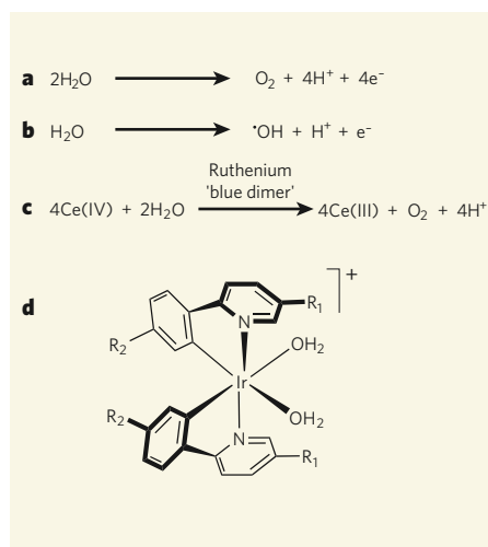
Figure 1 | Catalytic water oxidation.
